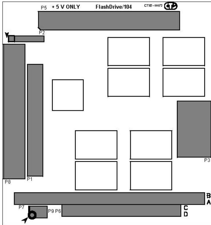
Figure 1: FlashDrive/104 Layout
