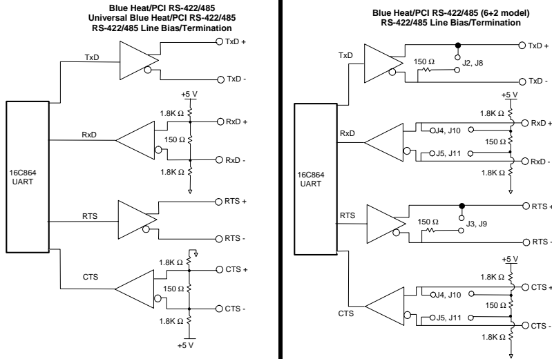
Figure 12: Partial schematic: Blue Heat/PCI RS-422/485; Universal Blue Heat/PCI RS-422-485
